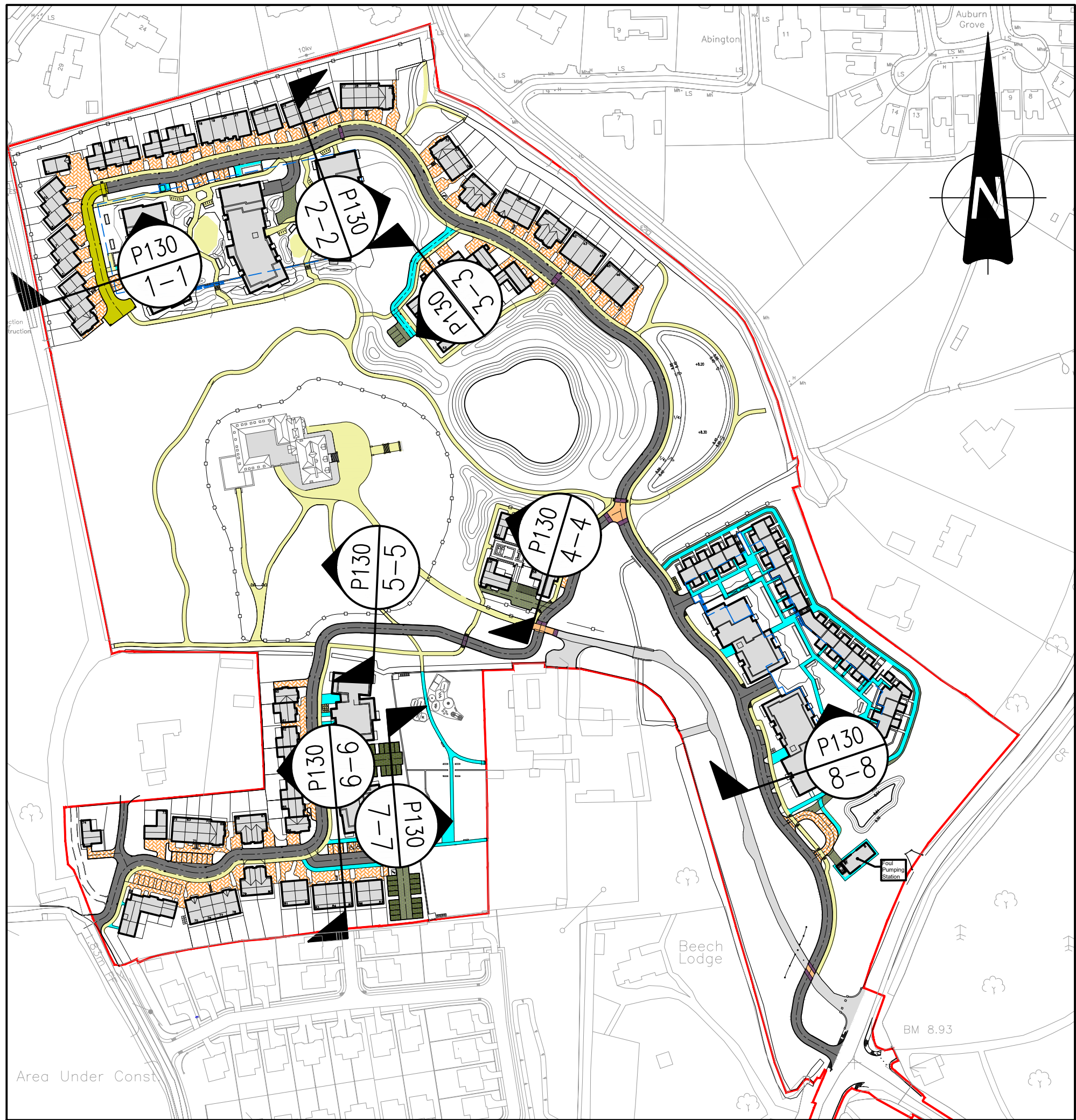
SECTION LOCATION PLAN SCALE 1:2000
